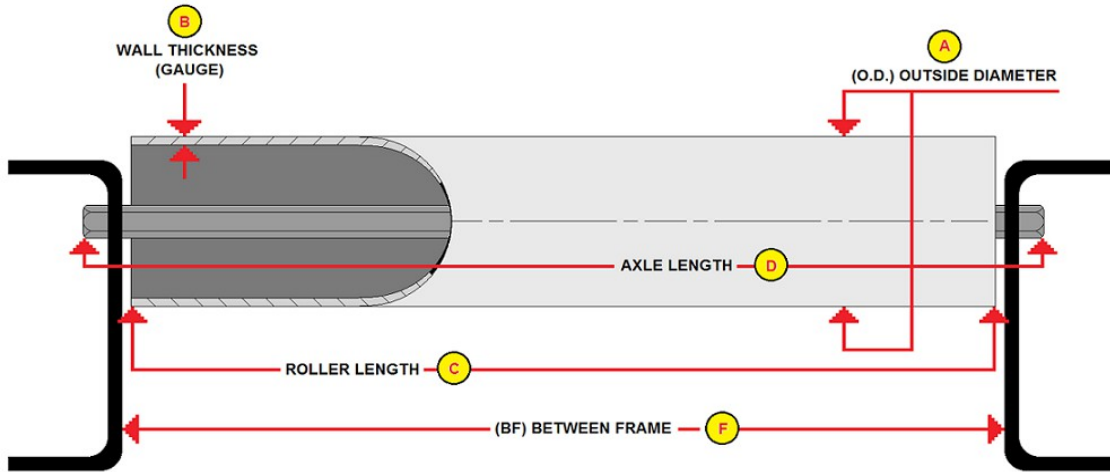
TYPICAL CROSS SECTION (Standard Frame)
